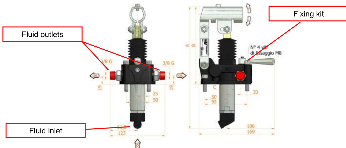
Fig.5.1: Hand pump - installation on tank
